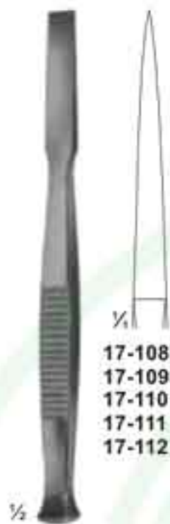
17-108 - 112 Osteotomes 140 mm
